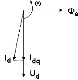
Fig.3. Phasor diagram \Phi_e - flux generated by the excitation current ; I_d - actual fault current; I_{dq} - fault current in the quadrature; U_d - voltage induced in the faulty sheets
