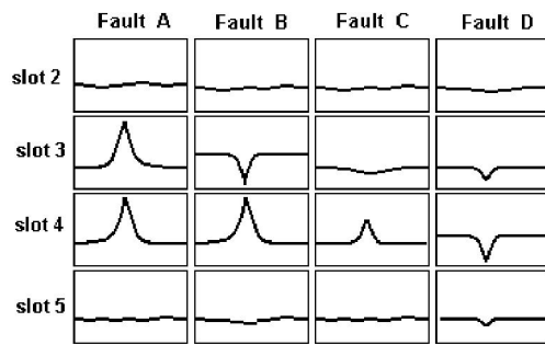
Fig.5. Basic forms of the Chattock signal
