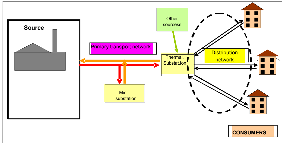
Fig. 1 DH - District Heating - Principle Scheme
