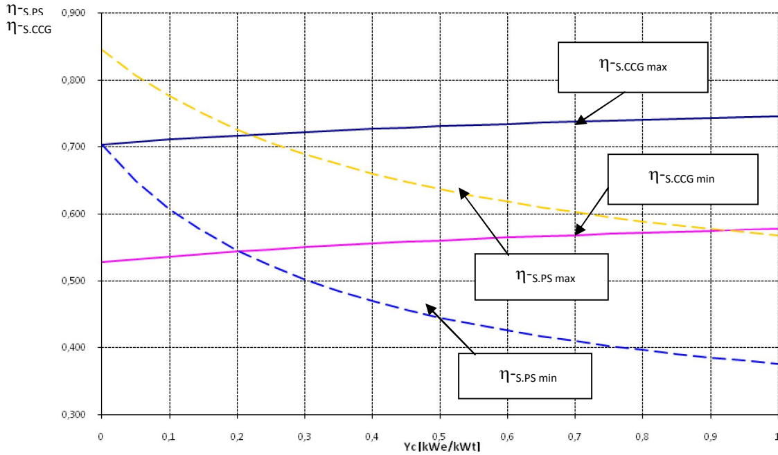
Fig. 5 Variation domains of \eta_{SPS} and \eta_{SCCG} function of y_c ( y_c=0,05 - 1,0 \text{ kWh}_e/\text{kWh}_t ), for limited values of \eta_{STDC}^Q , \eta_{SPEE} and \eta_{ICCG} .
