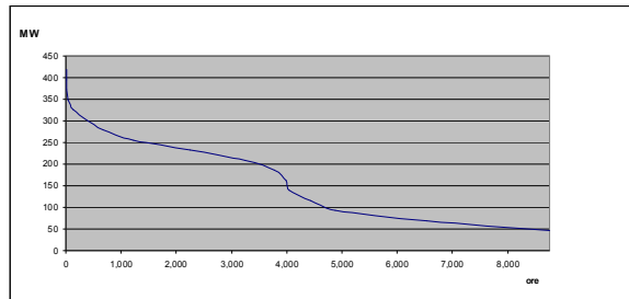
Fig.2 Annual consumption duration curve for thermal energy
