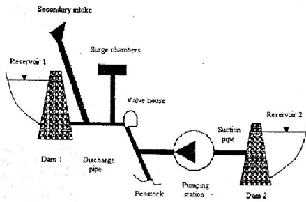
Fig. 1. The forward part of a hydro power system
