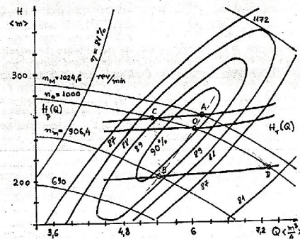
Fig. 3. A Sequence of the Characteristics Curves of the Two Centrifugal Pumps in Parallel.
