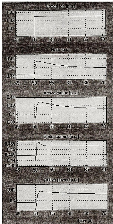
Fig. 6. The transients on the Hydro-Generator Side
