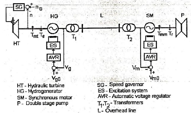
Fig. 5. The Simulated Power System
