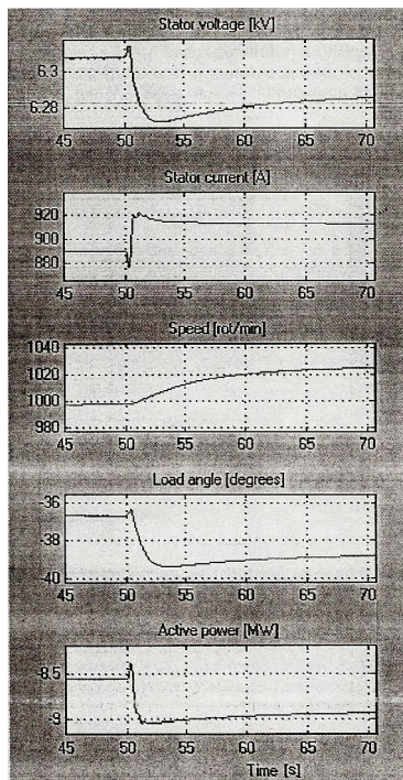
Fig. 7. Synchronous Motor Transits
