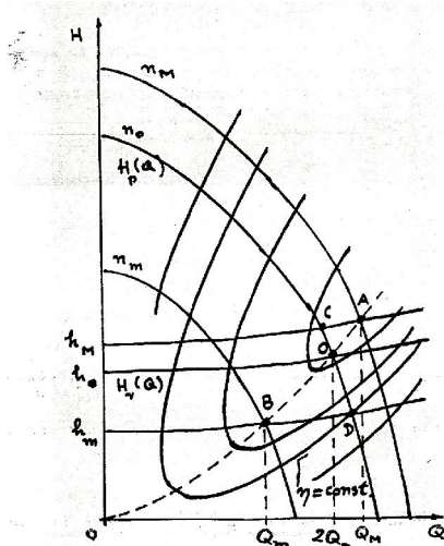
Fig. 4. Explanatory Plotting Head-Capacity-Speed Efficiency of the Pumps within the network
