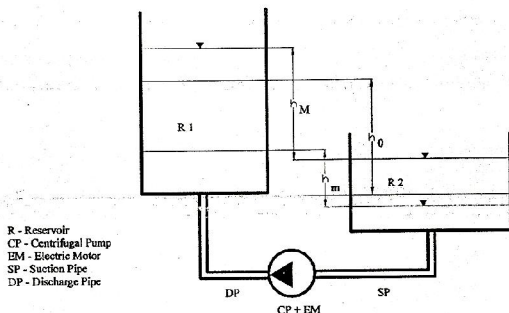
Fig. 2. Essential elements of a Hydraulic Pumping System
