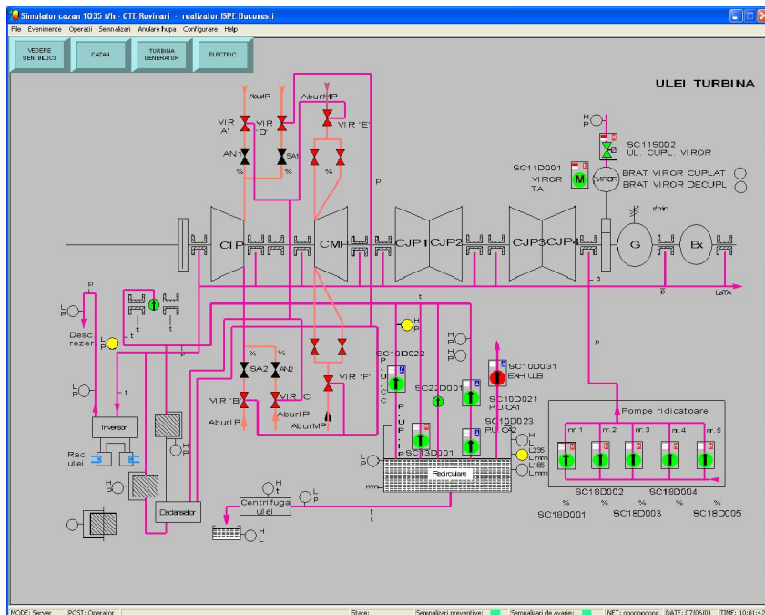
Fig.4. Turbine oil circuit diagram – 330 MW group simulator.
