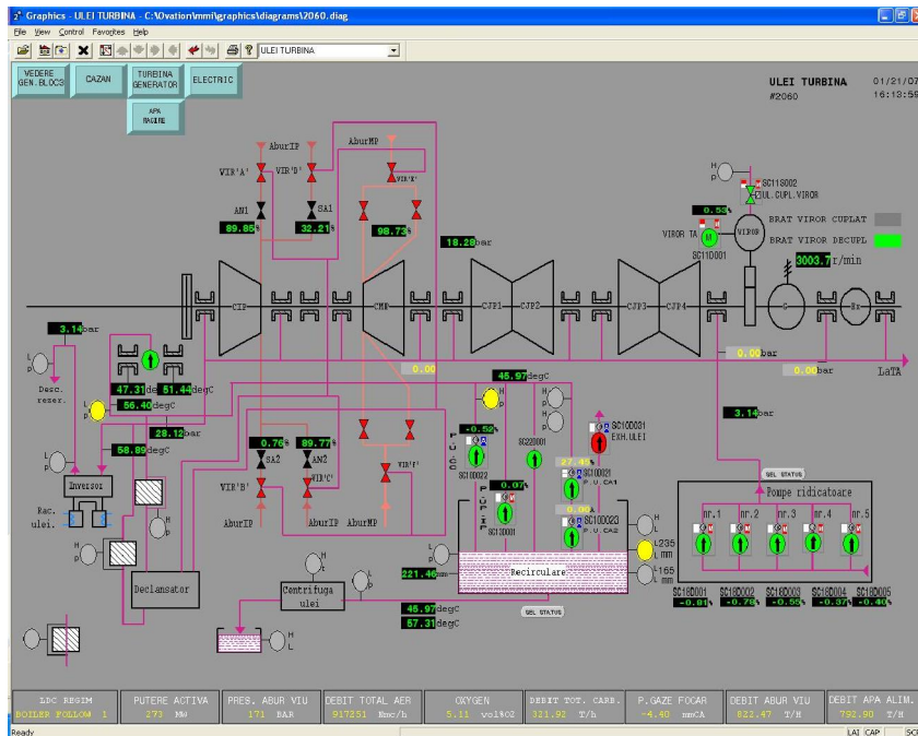
Fig.3. Turbine oil circuit diagram– Ovation system.
