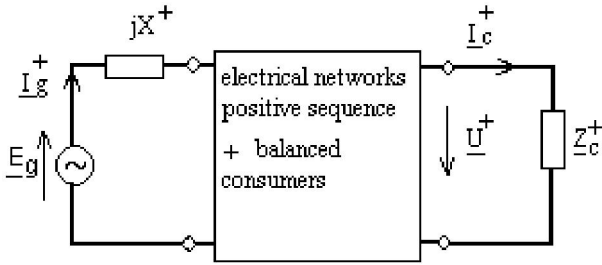
Fig.2. Positive sequence structure of considered electrical network.
