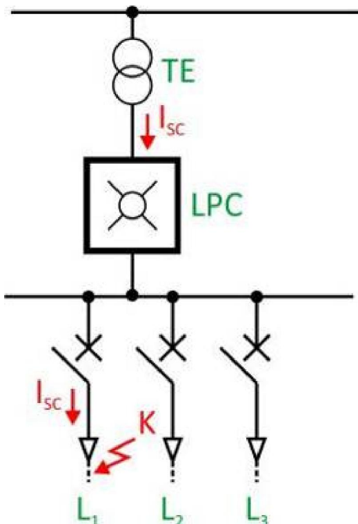
Fig. 4. Distribution scheme with one transformer
